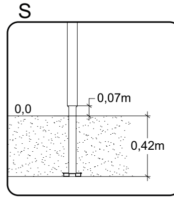
S Sunken Foundation 8113302
